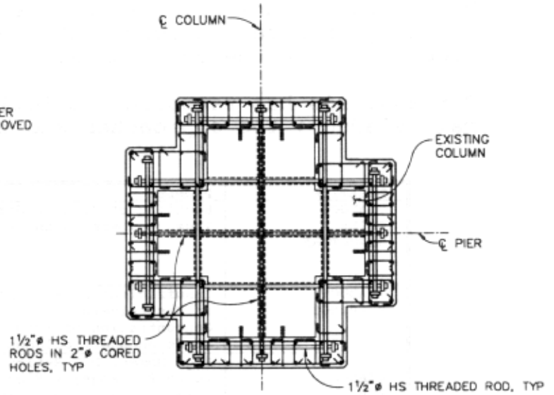
PIER SECTION
