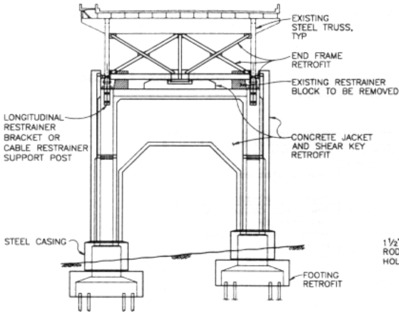
TYPICAL SECTION PIERS 3-8
